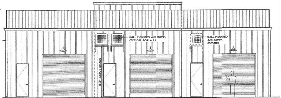
REAR ELEVATION 1/4" = 1'-0" SOUTH
